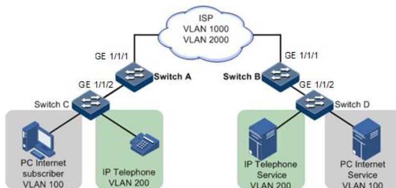
Figure 2-8 Selective QinQ networking
