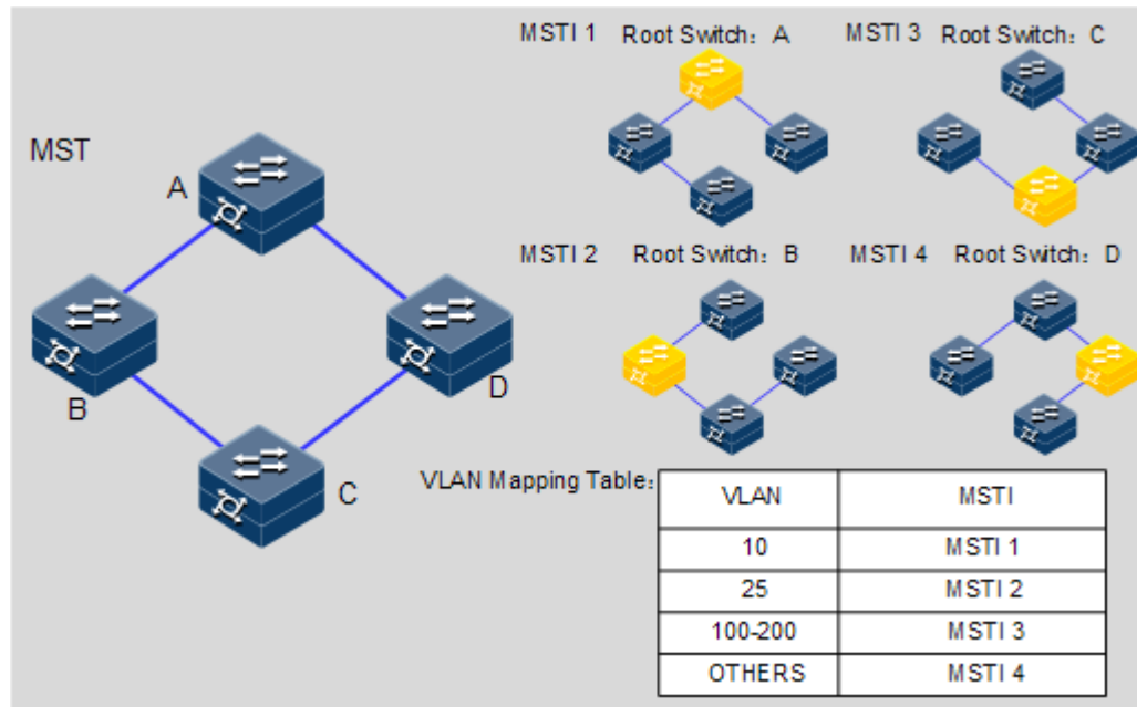
Figure 2-16 MSTI concepts
