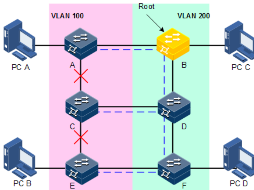
Figure 2-13 Failure to forward VLAN packets due to RSTP
