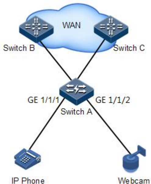
Figure 5-3 PoE switch power supply networking
