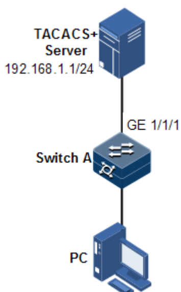
Figure 10-5 TACACS+ networking
