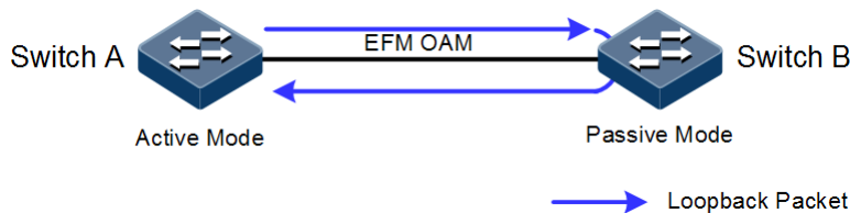
Figure 9-1 OAM loopback
