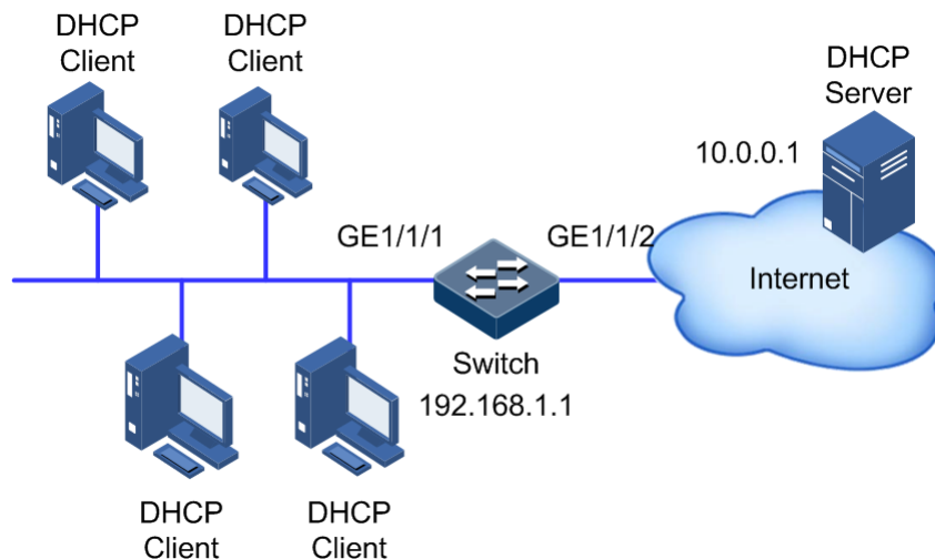
Figure 6-11 DHCP Relay networking
