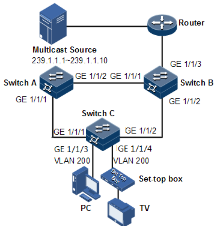
Figure 8-6 Ring network multicast networking
