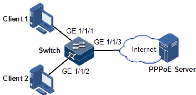
Figure 10-12 PPPoE+ networking
