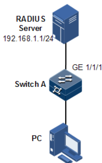
Figure 10-4 RADIUS networking
