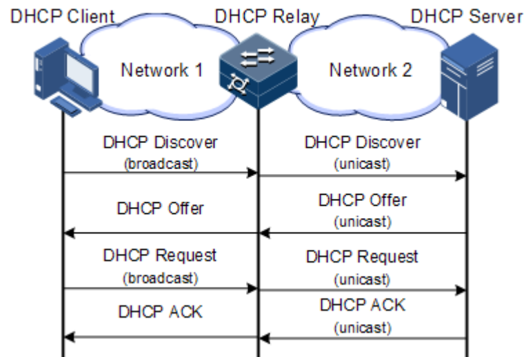
Figure 6-10 Typical application of DHCP Relay
