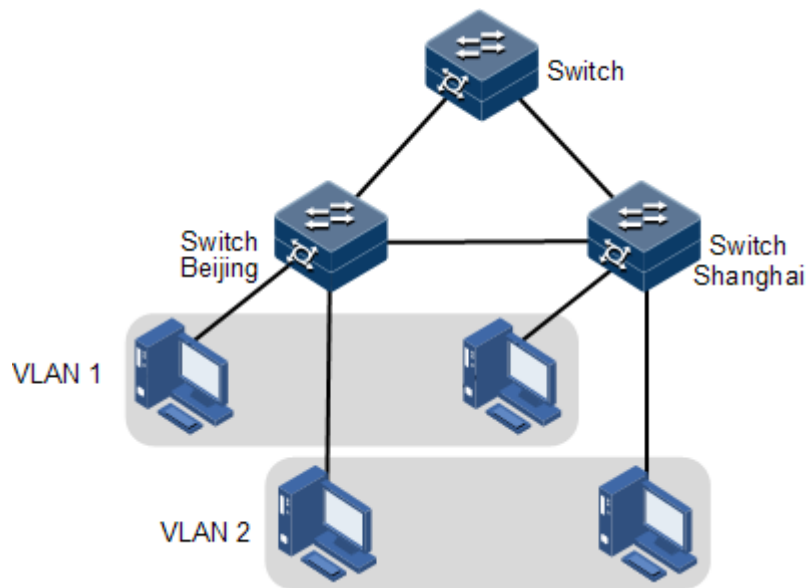
Figure 2-3 VLAN partition
