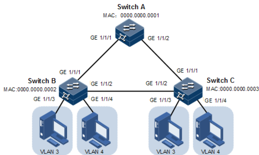
Figure 2-18 MSTP networking
