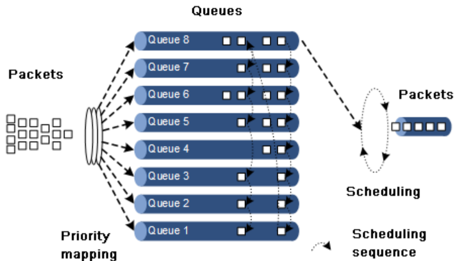
Figure 7-8 DRR scheduling
