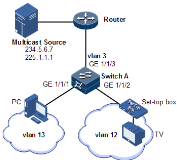
Figure 8-9 MVR networking
