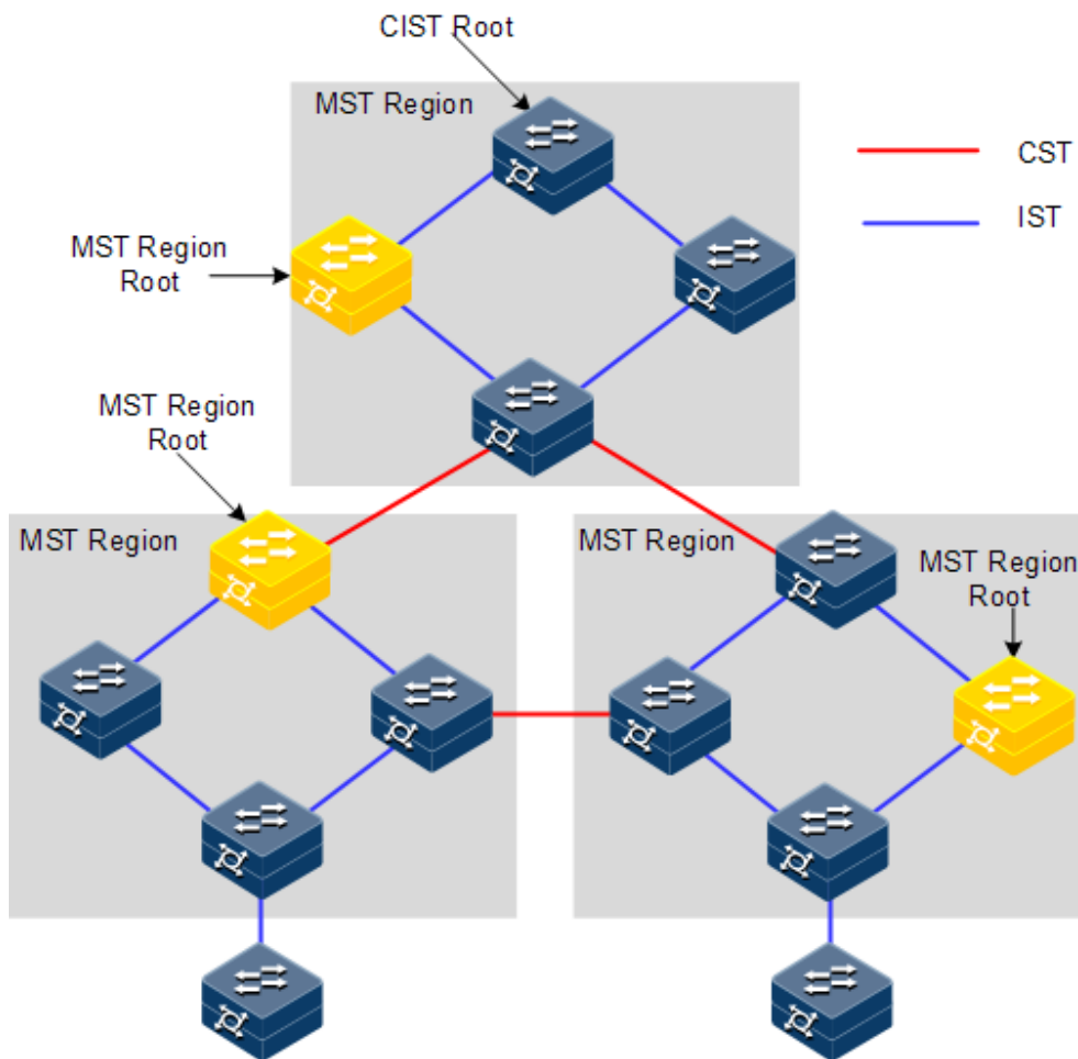
Figure 2-15 Basic concepts of the MSTI network
