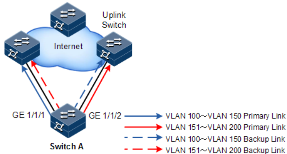
Figure 11-4 Networking with interface backup in different VLANs
