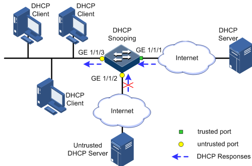
Figure 6-6 DHCP Snooping networking
