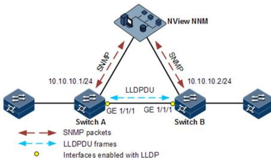
Figure 12-10 LLDP networking
