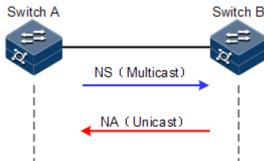
Figure 4-3 Principles of NDP address resolution
