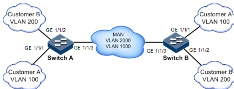
Figure 2-25 L2CP networking
