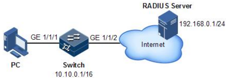
Figure 10-8 Dot1x networking
